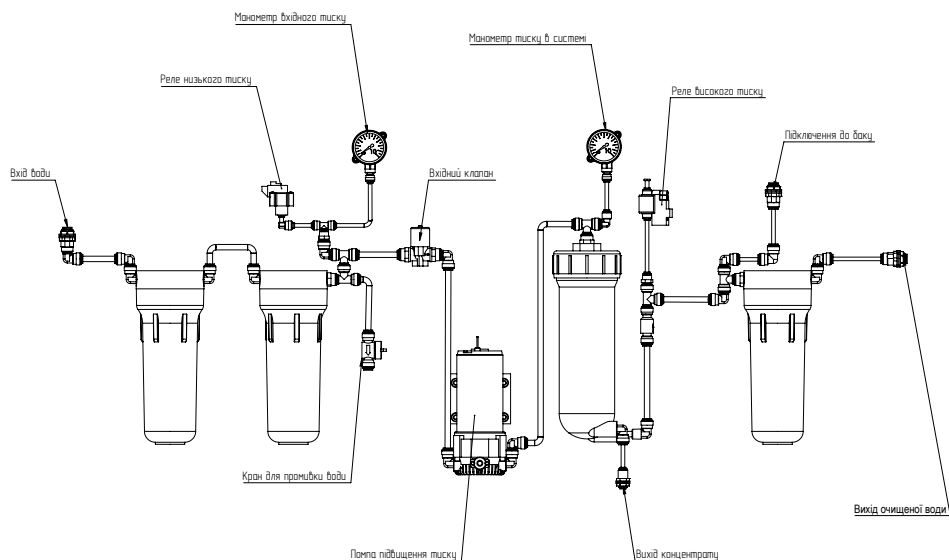
Figure 3. Robust 1500 ECO
