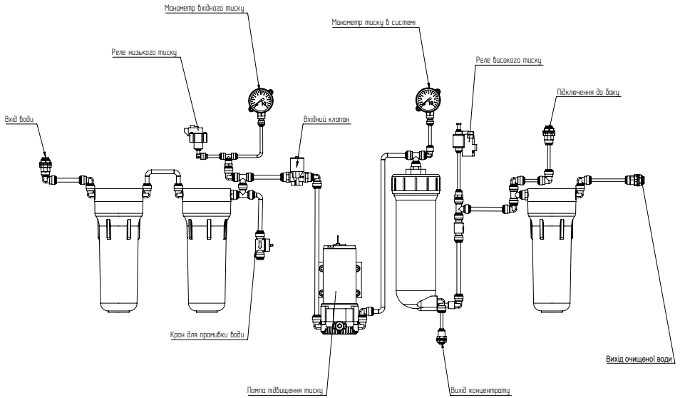
Figure 3. ROBUST 1500 ECO
